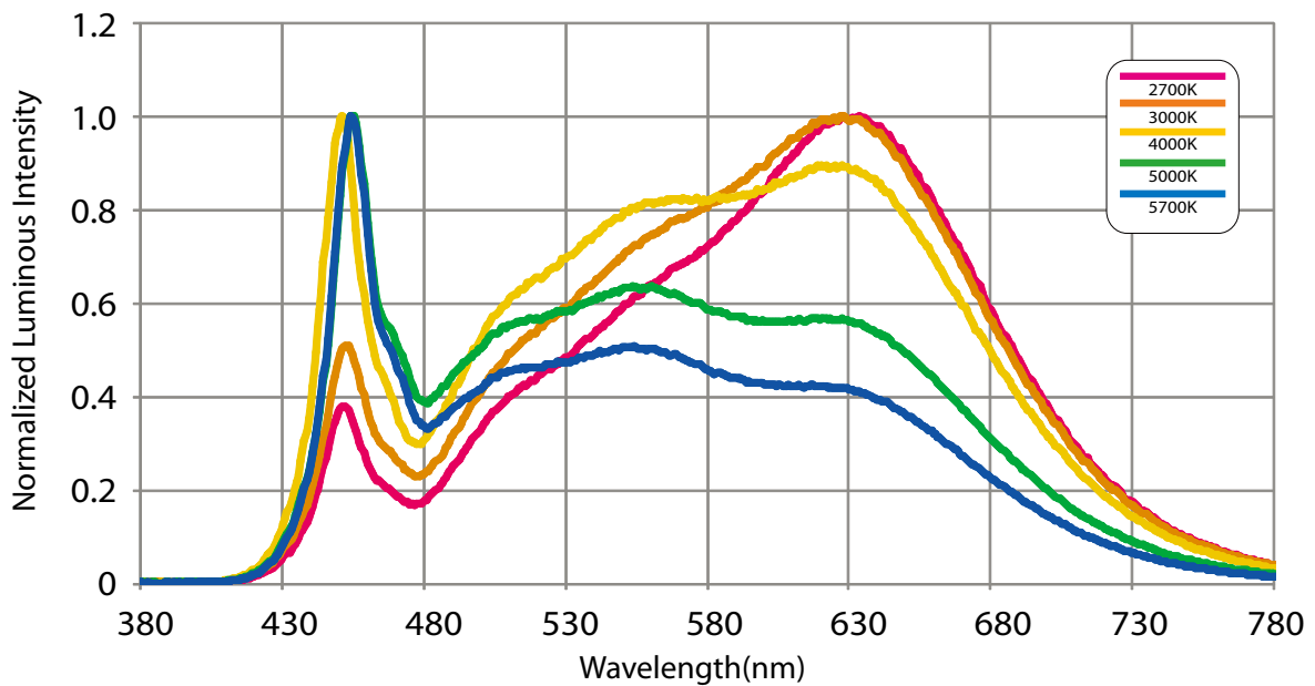
Color Spectrum(Tc=25°C,VAC=120V)_Ra 90
