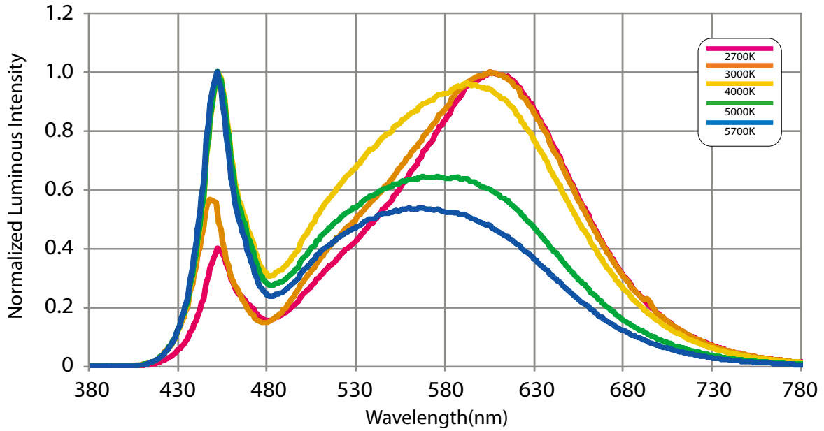
Color Spectrum(Tc=25°C,VAC=120V)_Ra 80
