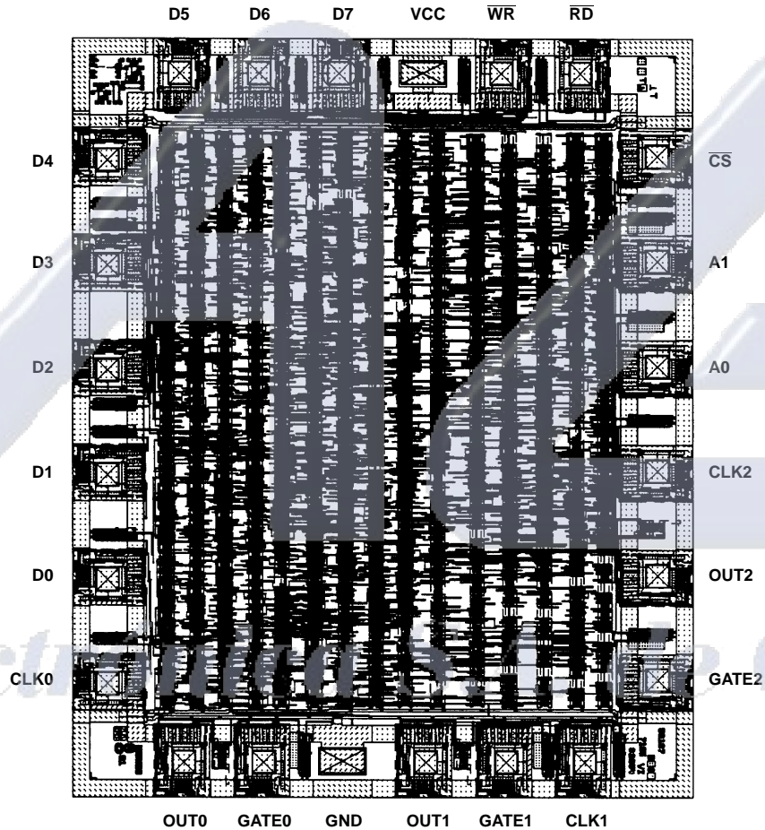
82C54
