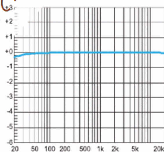
Figure 24. Frequency Response BTL mode, 3V, 80hm
