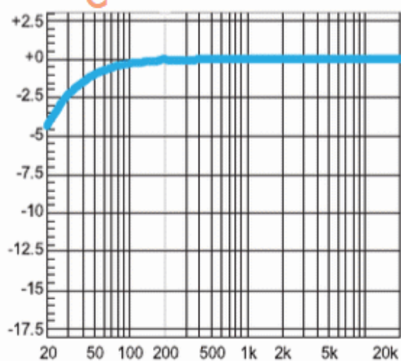
Figure 25. Frequency Response SE mode, 6V, 320hm, C5/C6=220uF
