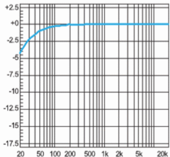
Figure 26. Frequency Response SE mode, 3V, 320hm, C5/C6=220uF
