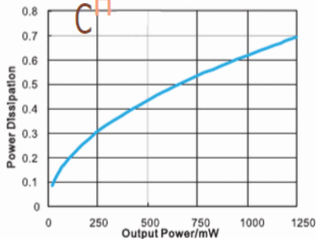
Figure 31. Power Dissipation vs. Output Power BTL mode, 5V, f=1\text{ kHz} , R_L=80\Omega , THD+N\leq 1\%
