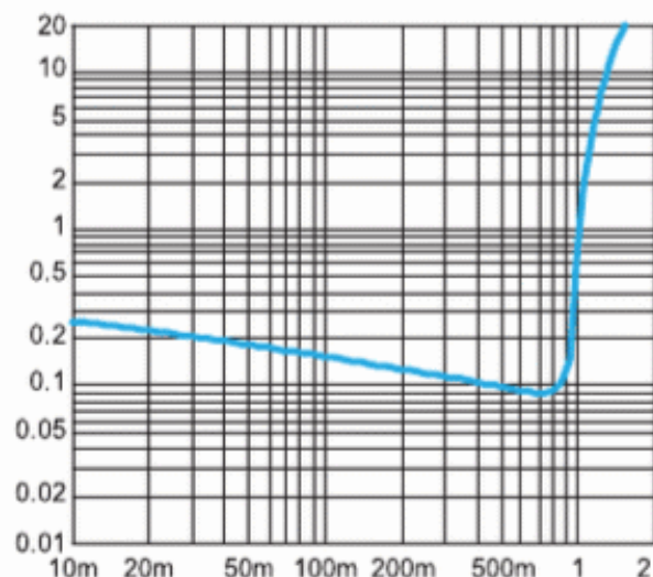
Figure 8. THD+N vs. Output Power BTL mode, 3V, 40hm, f=1 kHz
