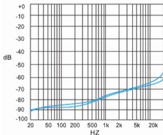
Figure 21. PSRR vs. Freq SE mode, 6V, 320hm, 200mVpp Input unterminated
