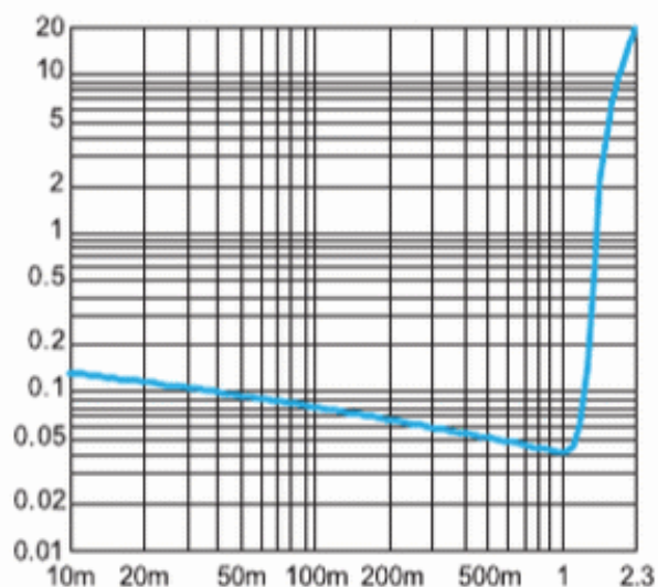
Figure 3. THD+N vs. Output Power 6V, 80hm, BTL at f=1 kHz
