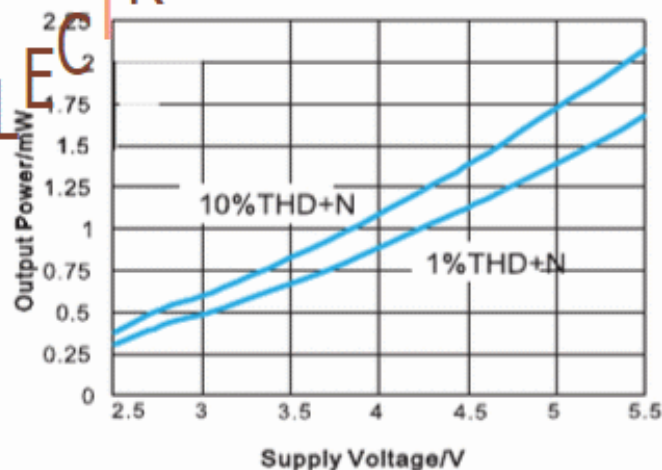
Figure 30. Output Power vs. Power Supply BTL mode, f=1\text{ kHz} , R_L=8\text{ }\Omega
