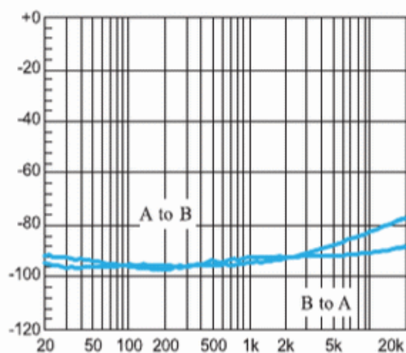
Figure 27. Crosstalk BTL mode, 6V, 80Ω, P_o=1W
