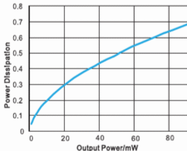
Figure 32. Power Dissipation vs. Output Power SE mode, 5V, f=1\text{ kHz} , R_L=320\Omega
