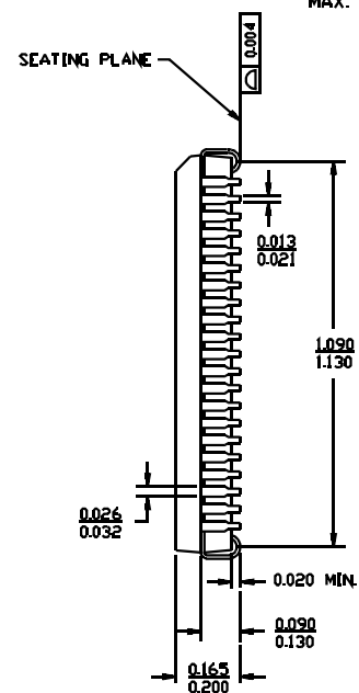
DIMENSIONS IN INCHES MIN. MAX.
