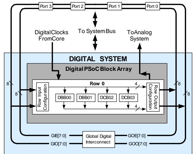
Figure 2. Digital System Block Diagram
