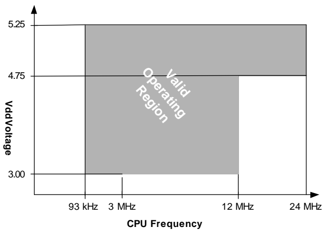
Figure 6. Voltage versus CPU Frequency
