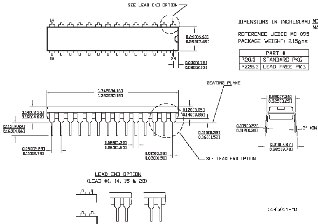
Figure 4-1. 28-Lead (300-Mil) Molded DIP
