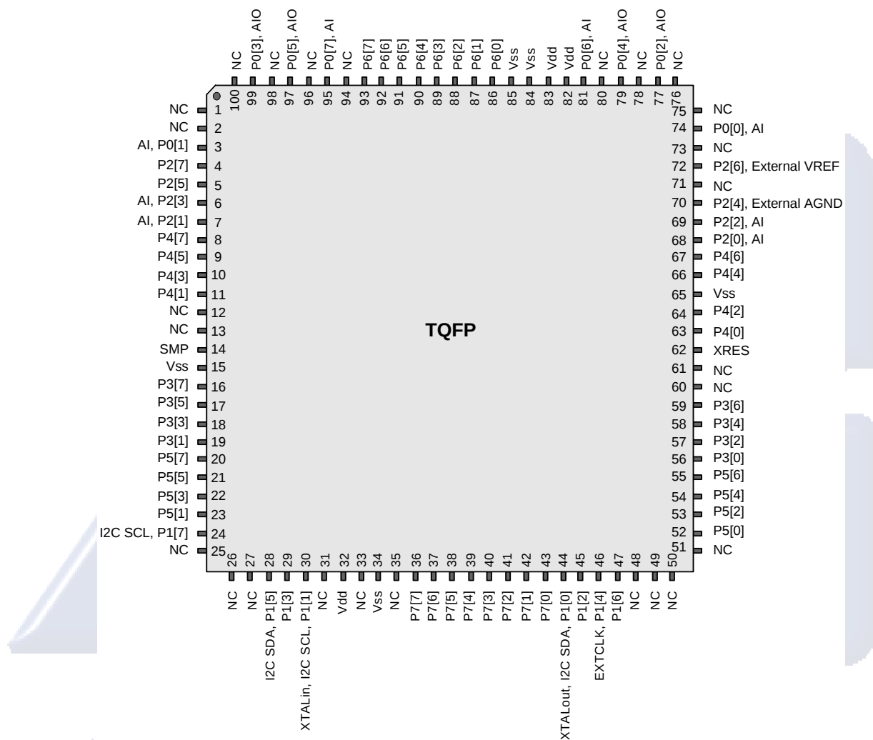
CY8C29866 100-Pin PSoC Device
