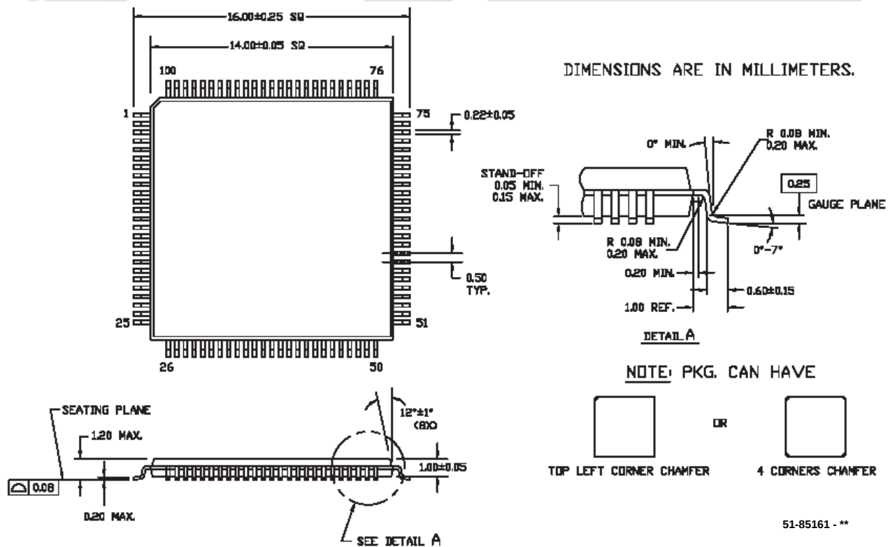
Figure 4-7. 100-Lead TQFP
