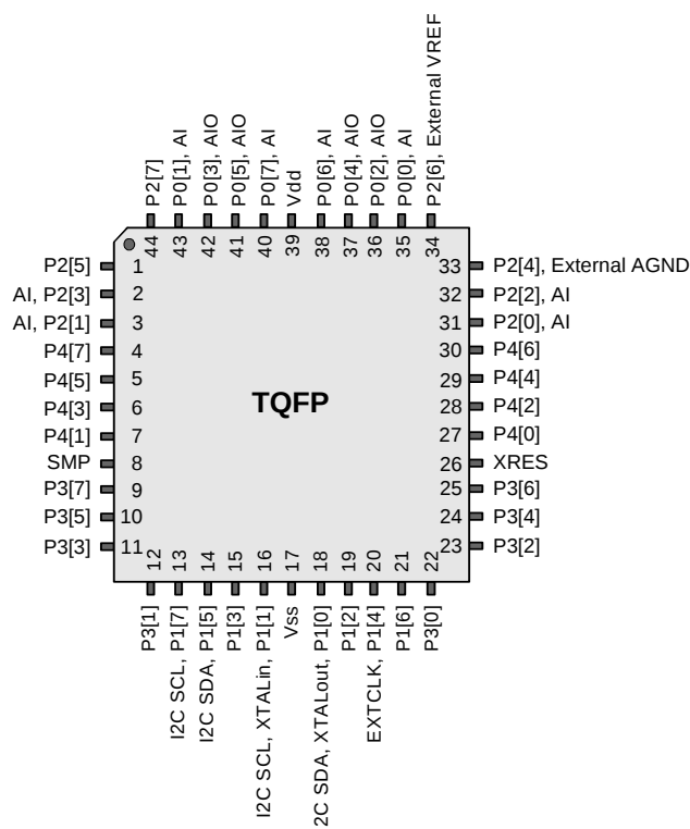
CY8C29566 44-Pin PSoC Device
