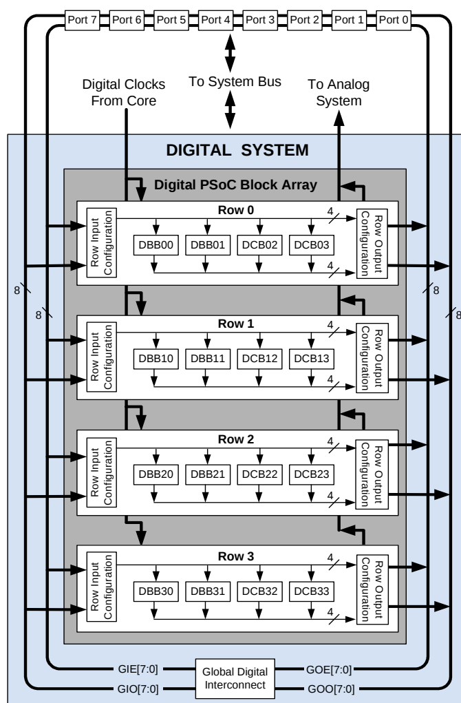
Digital System Block Diagram
