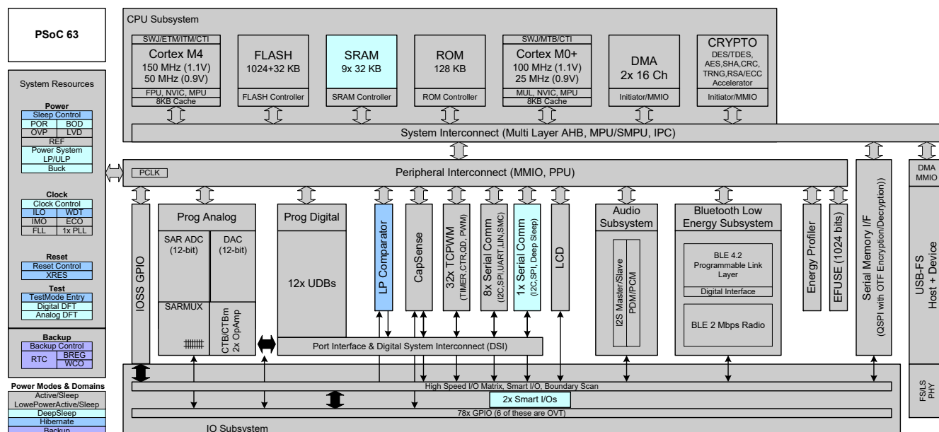
Figure 3. Block Diagram
