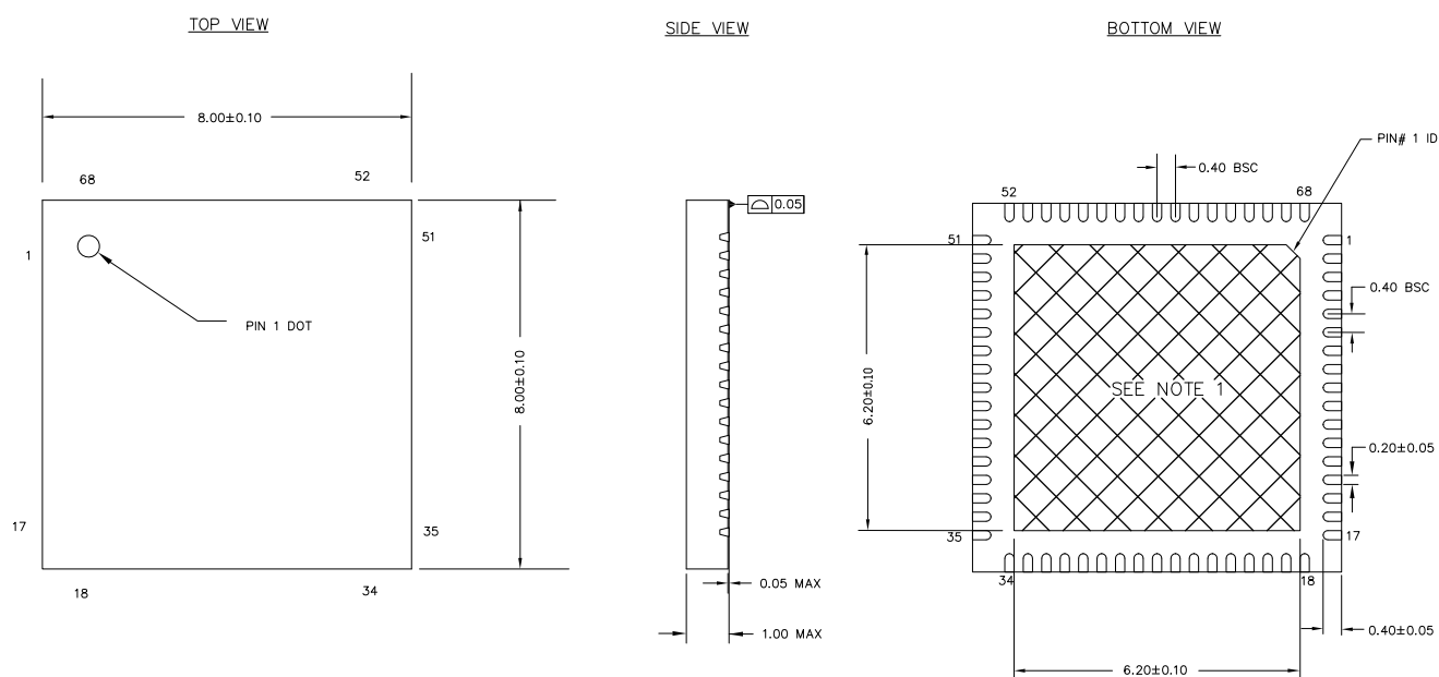
Figure 12. 68 QFN 8 × 8 × 1 mm
