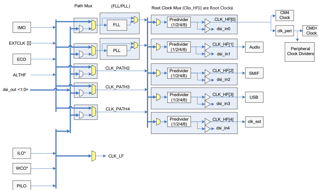
Figure 4. Clocking Diagram
