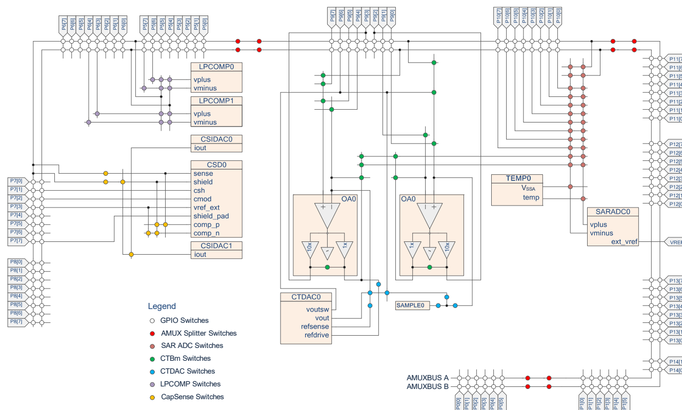
Figure 5. Analog Subsystem
