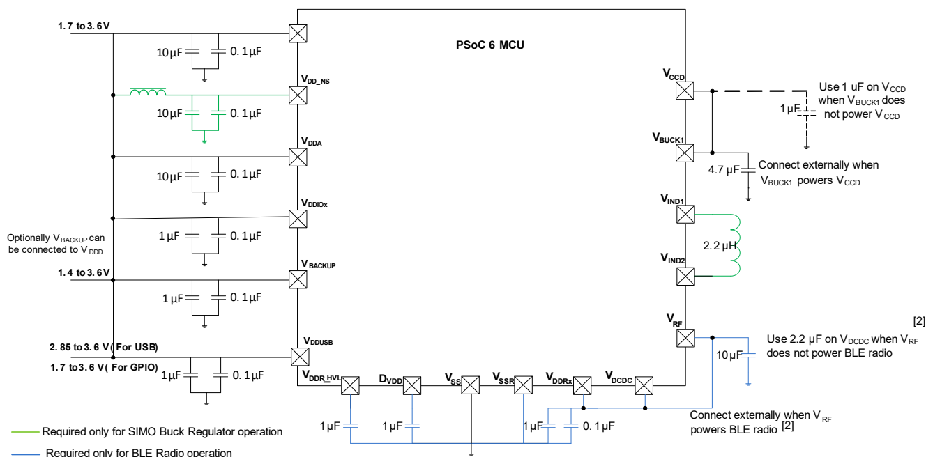
Figure 8. Power Connections
