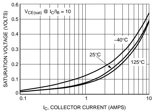
Figure 6. D45H11 ON-Voltage
