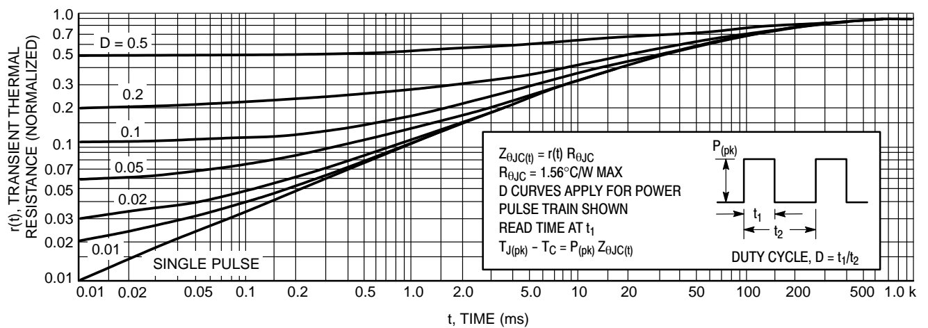
Figure 11. Thermal Response
