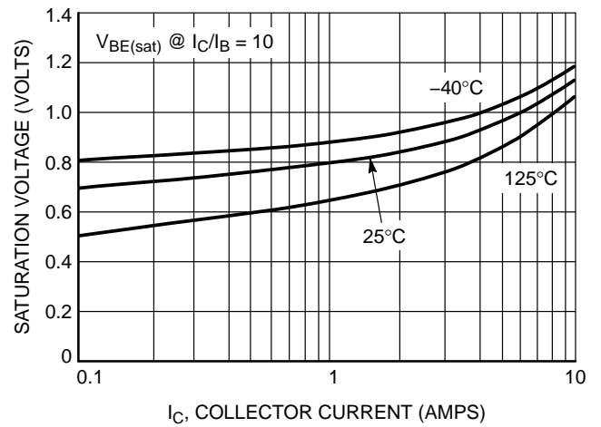
Figure 8. D45H11 ON-Voltage
