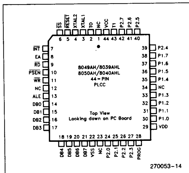
Figure 4. Pad Configuration
