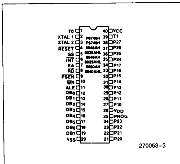
Figure 3. Pin Configuration
