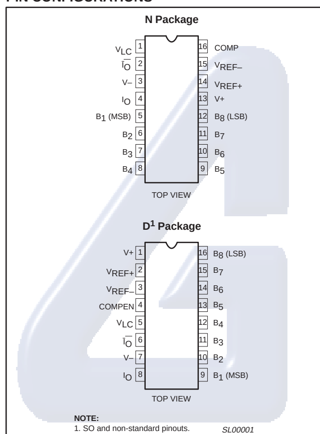
Figure 1. Pin Configuration
