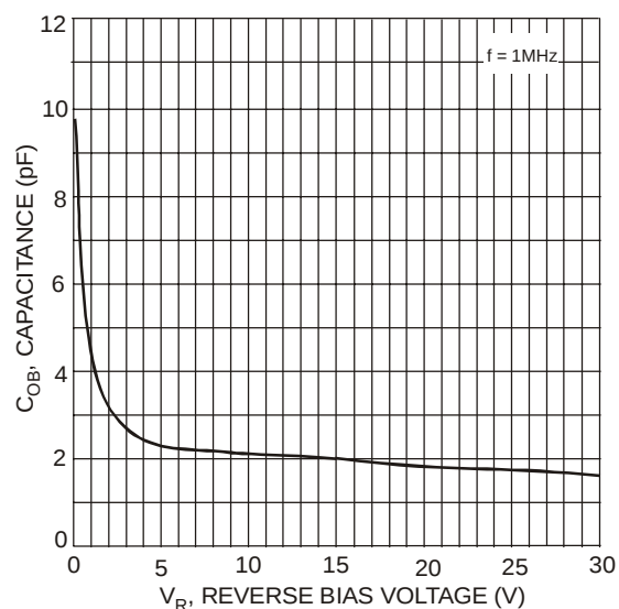
Fig. 4 Output Capacitance
