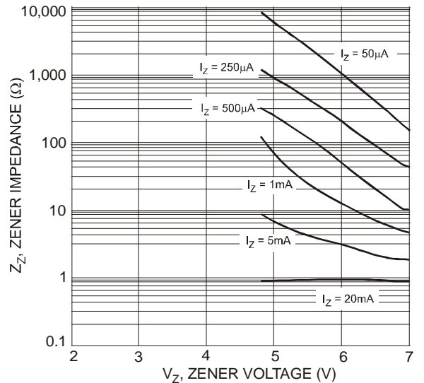
Fig. 11 Typical Zener Impedance Characteristics, DDZ9689S - DDZ9692S
