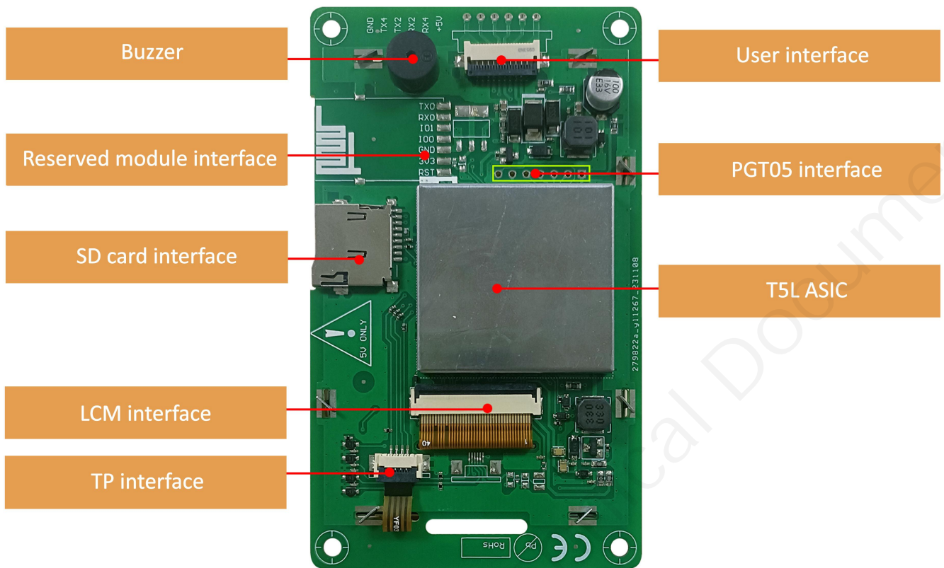
Hardware interface
