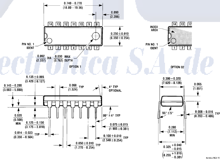
Molded Dual-In-Line Package (N) Order Number DS1489N or DS1489AN NS Package Number N14A
