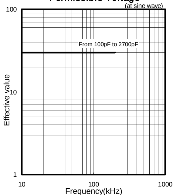
Permissible Voltage
