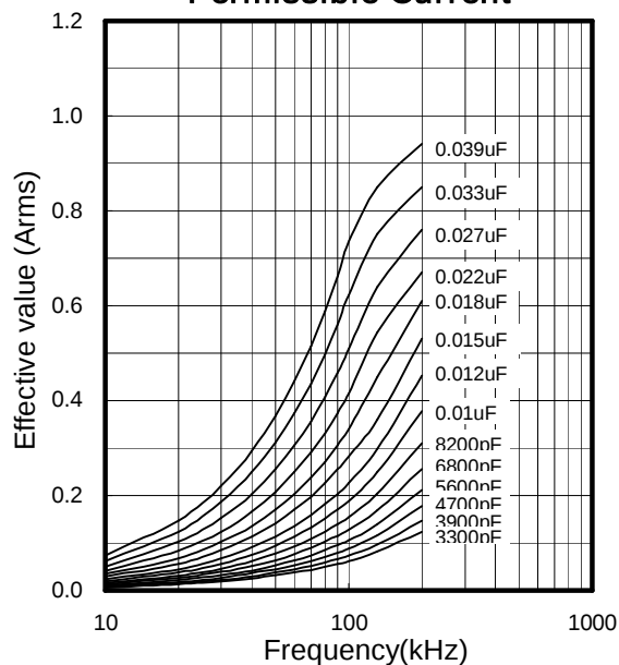
Permissible Current
