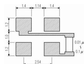
Figure 2) Land Pattern
