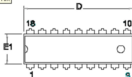
18-Lead Plastic Dual in line (PDIP) — 300 mil
