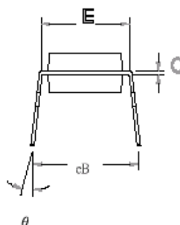
18-Lead Plastic Dual in line (PDIP) — 300 mil
