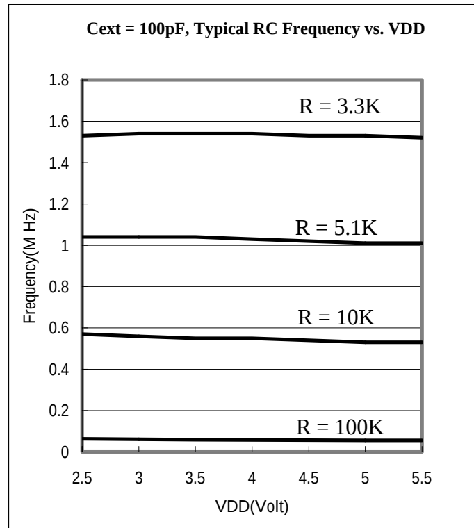
Fig. 24 Typical RC OSC Frequency vs. VDD (Cext= 100pF, Temperature at 25 °C)
