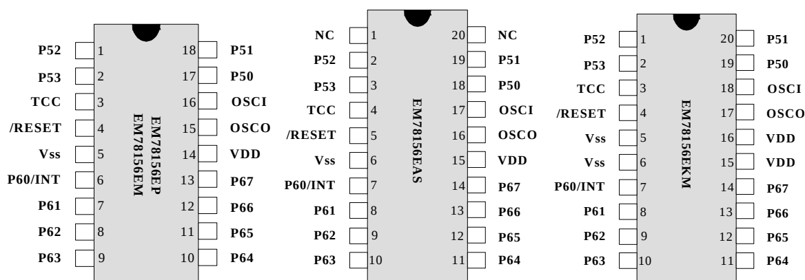
Fig. 1 Pin Assignment
