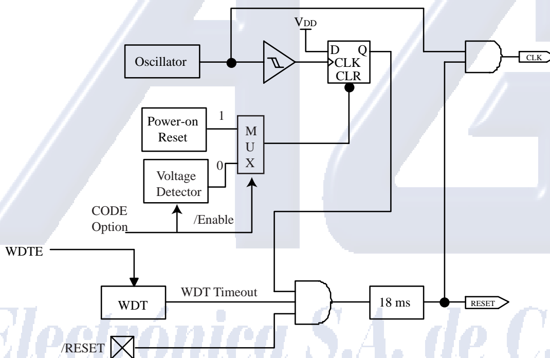
Fig. 9 Block diagram of Reset of controller
