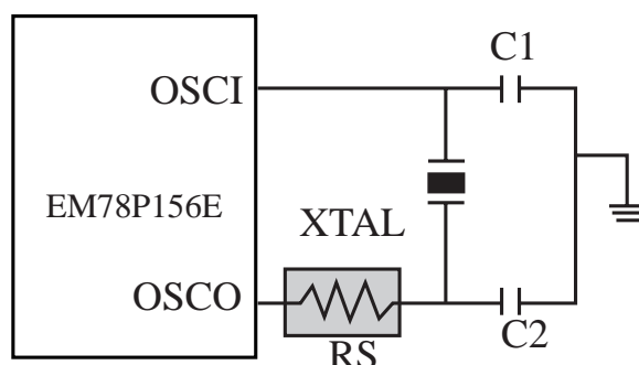
Fig. 12 Circuit for Crystal/Resonator
