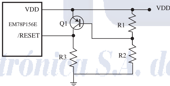
Fig. 16 Circuit 2 for the residue voltage protection
