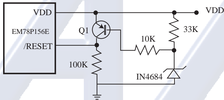
Fig. 15 Circuit 1 for the residue voltage protection
