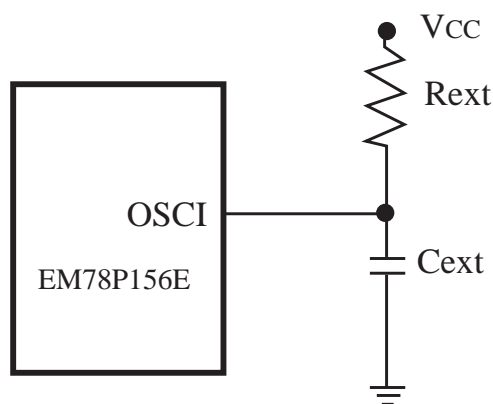
Fig. 13 Circuit for External RC Oscillator Mode
