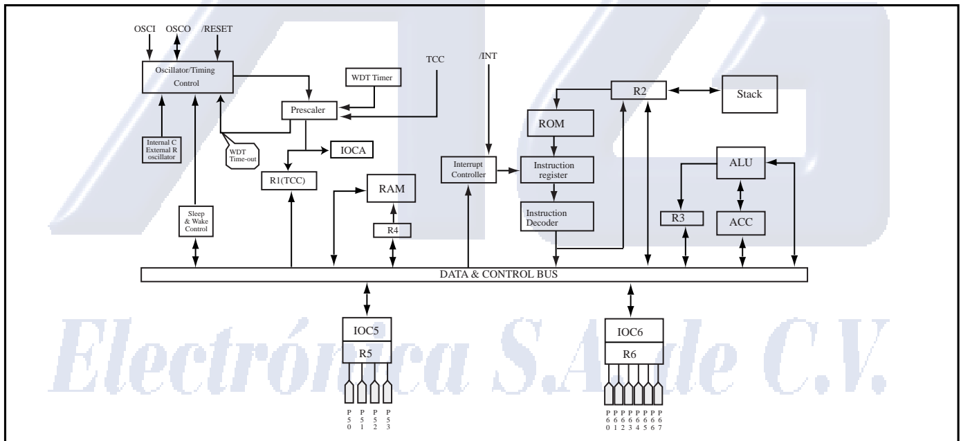
IV. FUNCTIONAL BLOCK DIAGRAM
