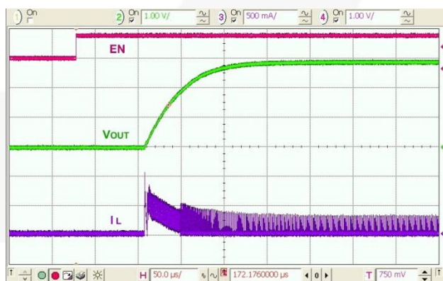
Figure 25. Startup, V_{OUT}=2.9\text{ V} , 50 \Omega Load
