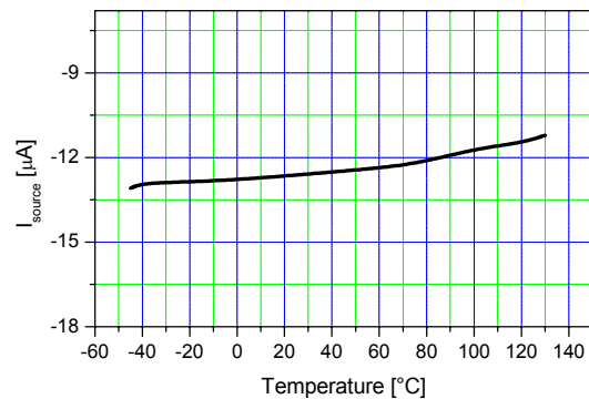
Figure 15. Output Source Current vs. Temp.
