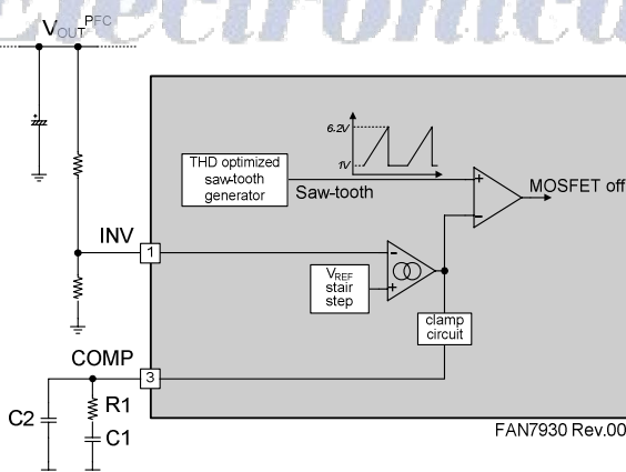
Figure 30. Control Circuit
