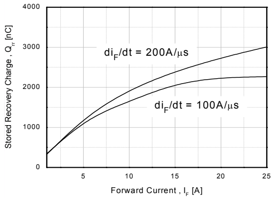
Figure 20. Stored Charge
