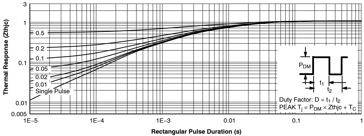
Figure 22. Transient Thermal Impedance of Diode
