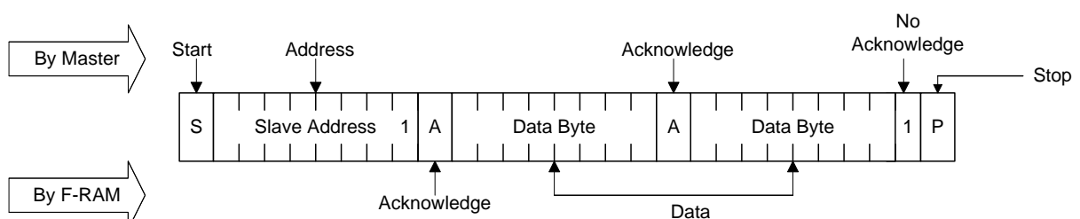
Figure 11. Sequential Read
