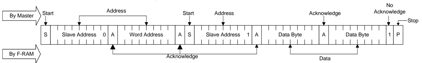
Figure 12. Selective (Random) Read
