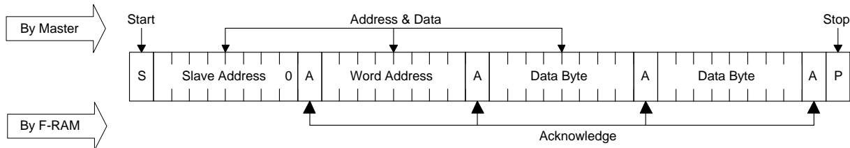
Figure 9. Multi-Byte Write
