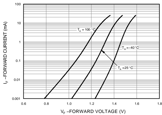
Figure 14. Input Forward Current vs. Forward Voltage
