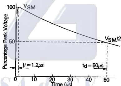
1.2/50 \mu\text{s} open-circuit waveform (Haefley Model P6T generator)
