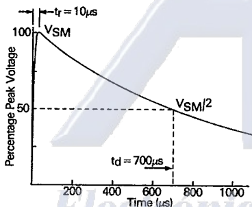
10/700 \mu\text{s} open-circuit waveform (Haefley Model P6T generator)
