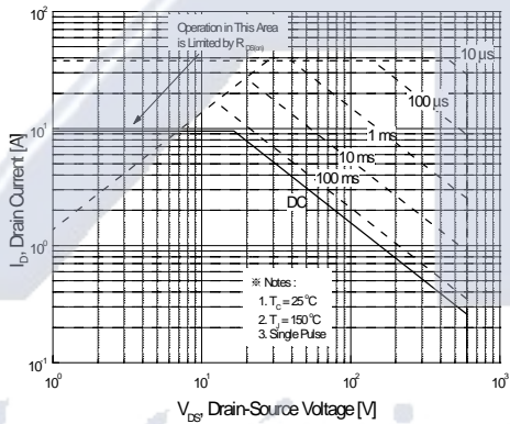
Figure 9-1. Maximum Safe Operating Area for FQP10N60C
