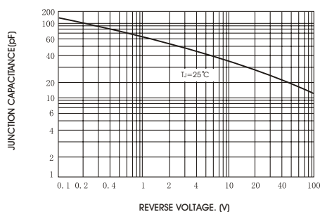
FIG. 4-TYPICAL JUNCTION CAPACITANCE
