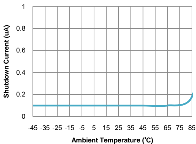
Figure 13. Shutdown Current vs. Ambient Temperature V_{IN}=12V , V_{SHDN}=2V , V_{OUT}=1V , L=1.5\mu H
