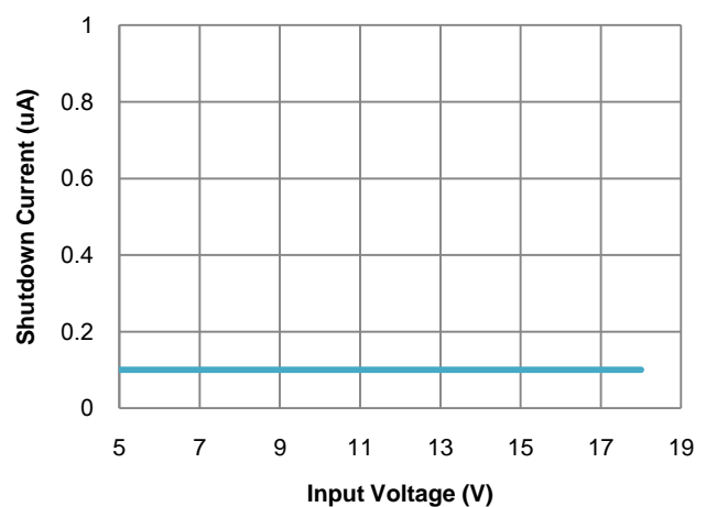
Figure 14. Shutdown Current vs. Input Voltage V_{IN}=12V , V_{SHDN}=2V , V_{OUT}=5V , L=3.3\mu H
