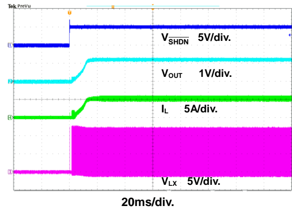
Figure 24. Startup Through \overline{SHDN} Waveform
