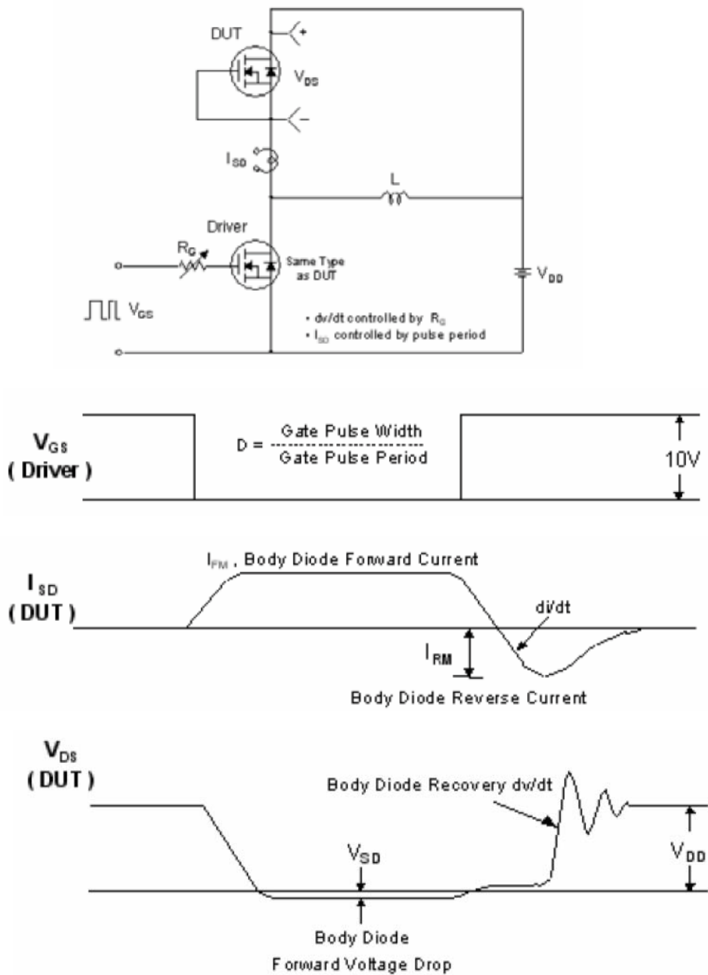
Peak Diode Recovery dv/dt Test Circuit and Waveform
