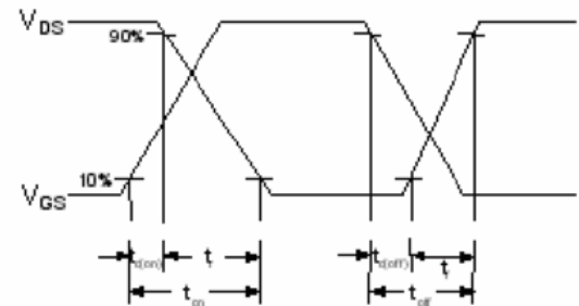
Resistive switch Test Circuit and Waveform
