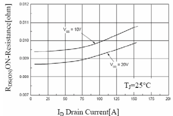
ON-Resistance Variation
