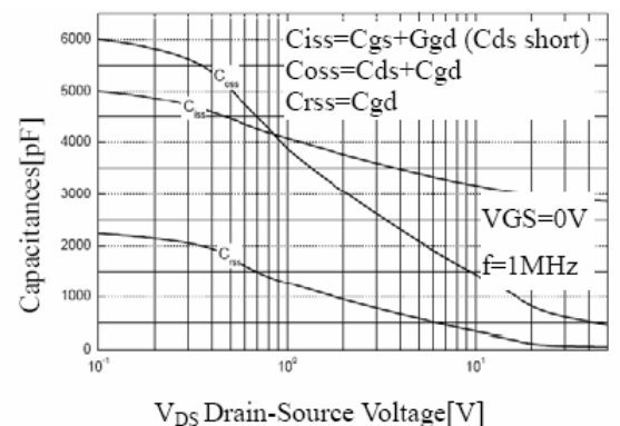
Capacitance Characteristics
