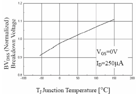
Breakdown Voltage Variation
