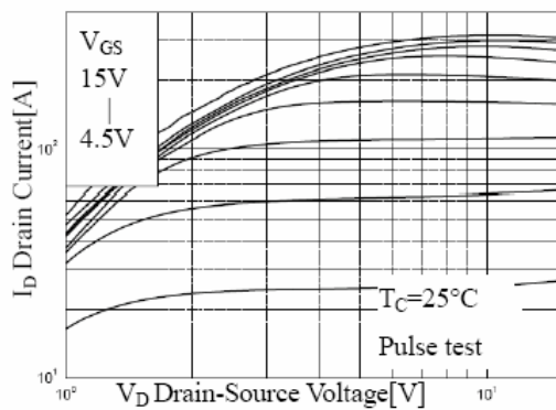
On-region Characteristics
