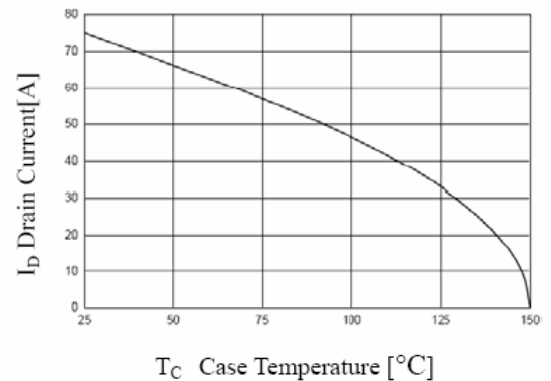
Maximum Drain Current
