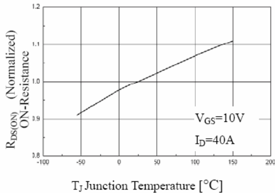
On-Resistance Variation
