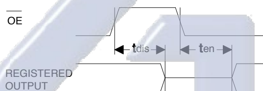
\overline{OE} to Output Enable/Disable
