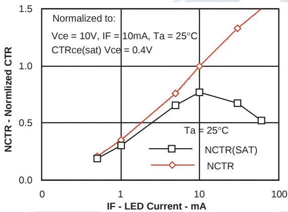
Figure 2. Normalized non-saturated and saturated CTR, T_A=25^\circ\text{C} vs. LED current
