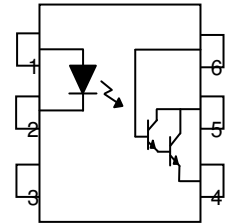
Pin Configuration
