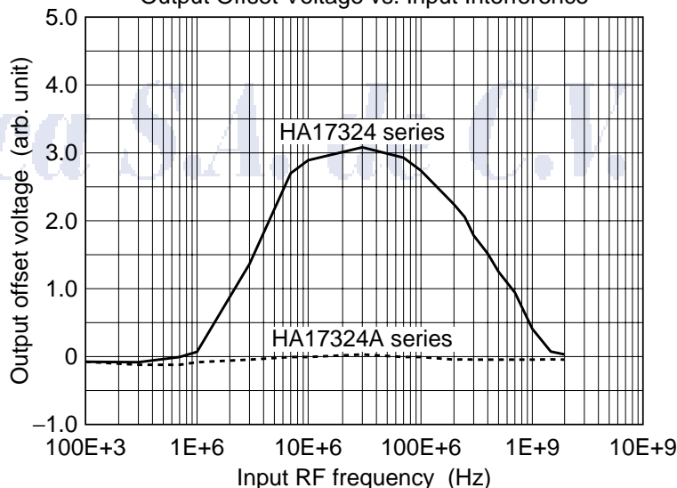
Output Offset Voltage vs. Input Interference
