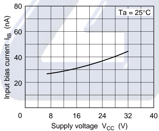
Input Bias Current vs. Supply Voltage
