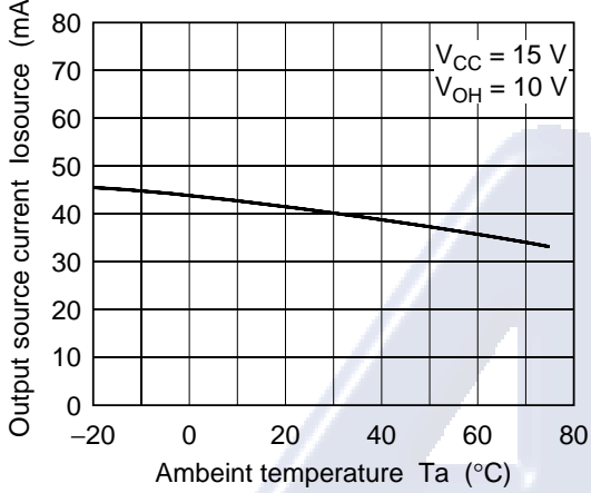
Output Source Current vs. Ambient Temperature
