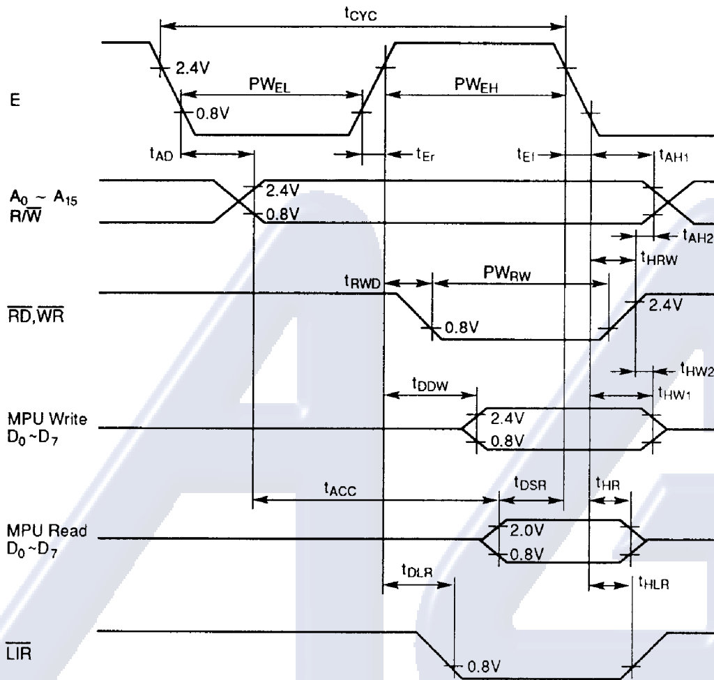
Figure 1 Bus Timing
