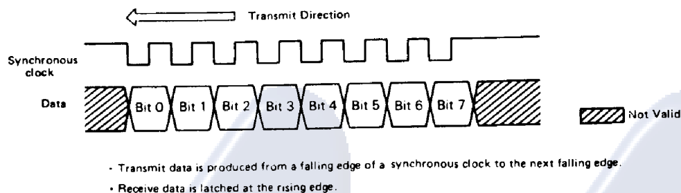
Figure 26 Clocked Synchronous Mode Format
