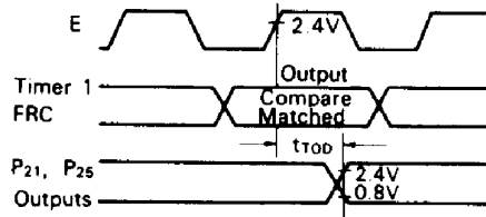
Figure 7 Timer 1 Output Timing
