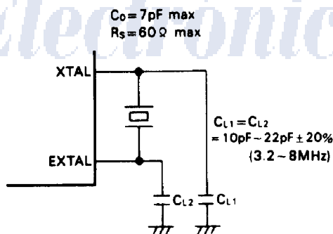
Figure 15 Connection Circuit
