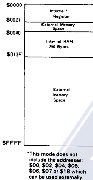
Figure 20 HD6303Y Memory Map
