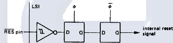
Figure 35 \overline{\text{RES}} circuit
