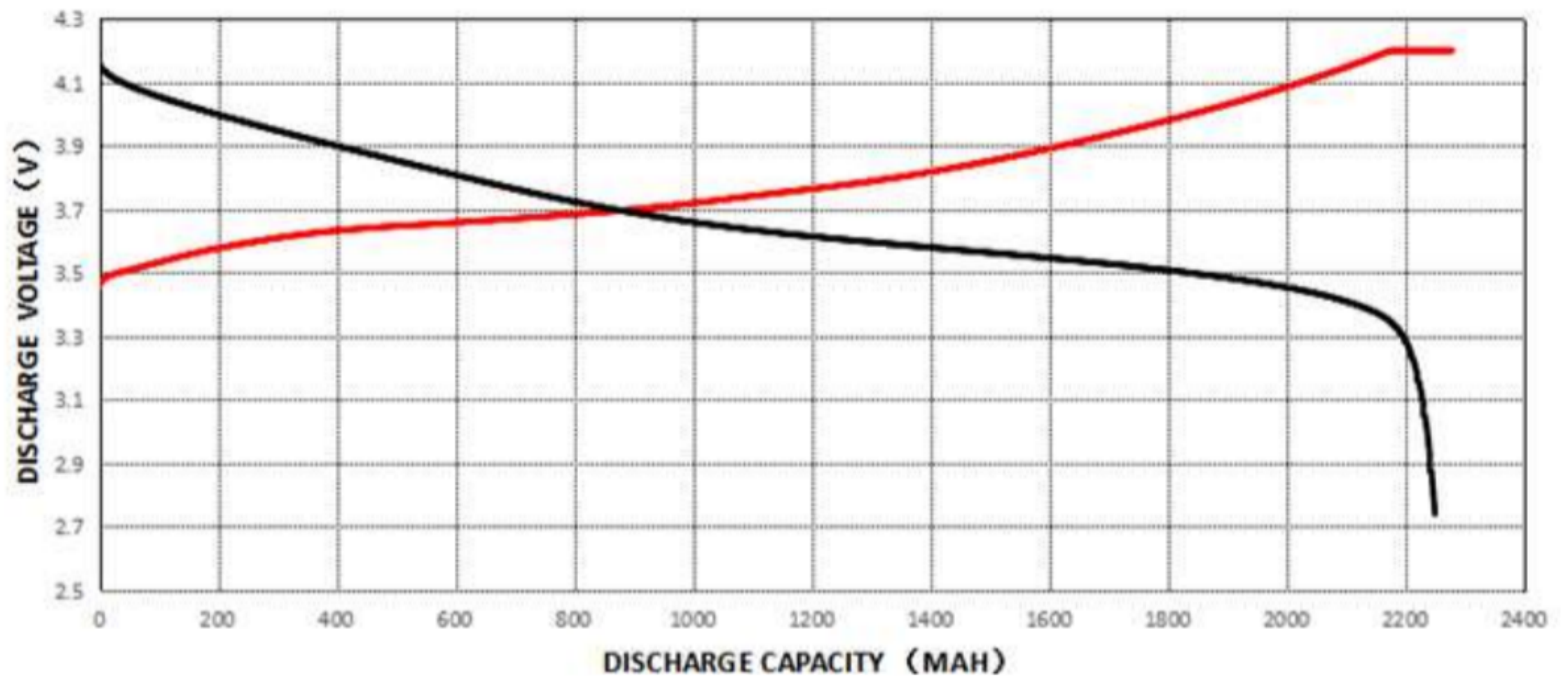
HDCNR18650-2200mAh-3.7 V (5C)
