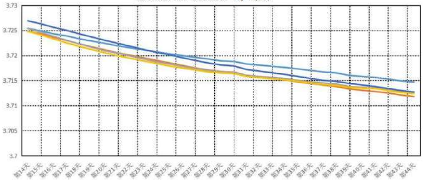
HDCNR18650-2600mAh-3.7V(3C)
