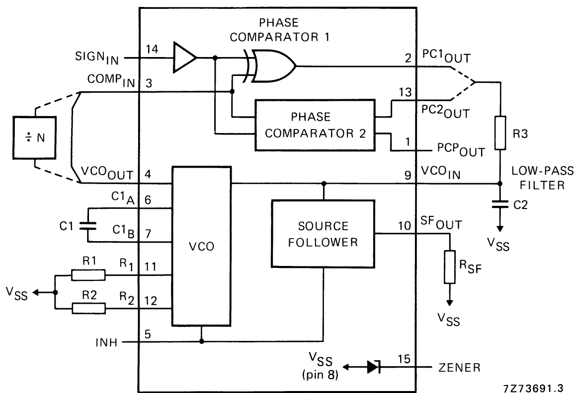
Fig.1 Functional diagram.
