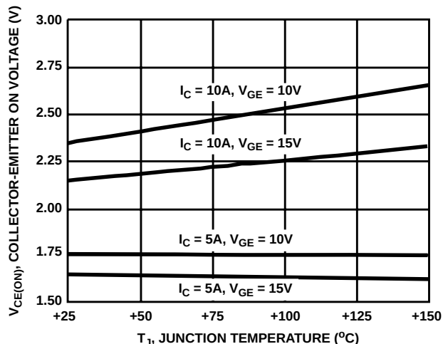
FIGURE 8. TYPICAL V_{CE(ON)} vs TEMPERATURE
