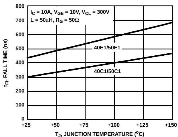
FIGURE 12. TYPICAL FALL TIME ( I_C = 10\text{A} )
