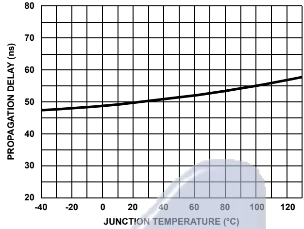
FIGURE 17. DISABLE TO LOWER ENABLE T_{DLE} PROPAGATION DELAY vs TEMPERATURE
