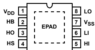
HIP2101 (SOIC, ESOIC) TOP VIEW
