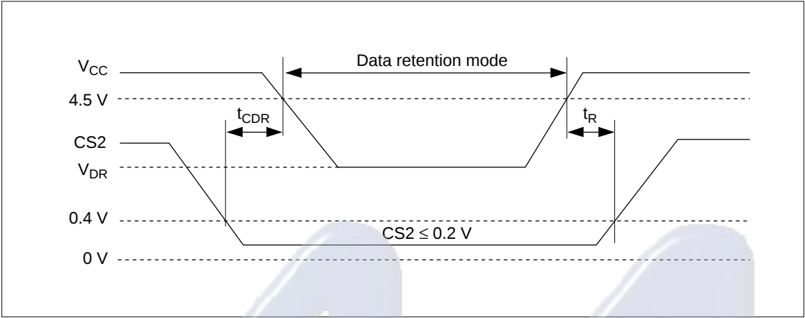
Low V CC Data Retention Waveform (2) (CS2 Controlled)
