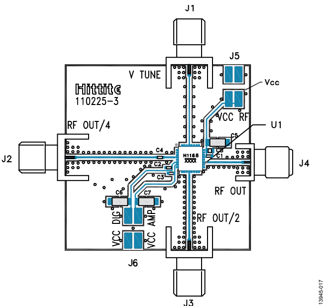
Figure 17. Evaluation PCB
