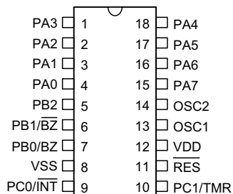
HT48R05A-1 - 18 DIP/SOP
