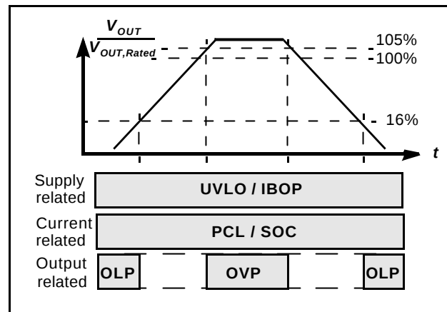
Figure 6 Protection Features
