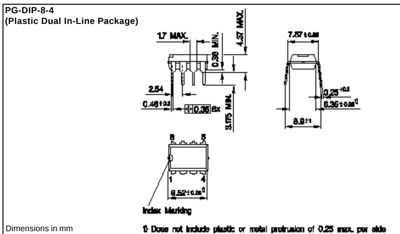
Figure 15 PG-DIP-8-4 Outline Dimension
