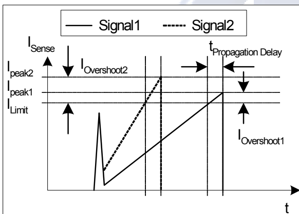
Figure 17 Current Limiting
