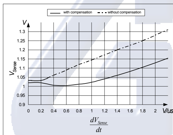
Figure 19 Overcurrent Shutdown
