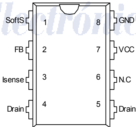
Figure 1 Pin Configuration P-DIP-8-6 (top view)
