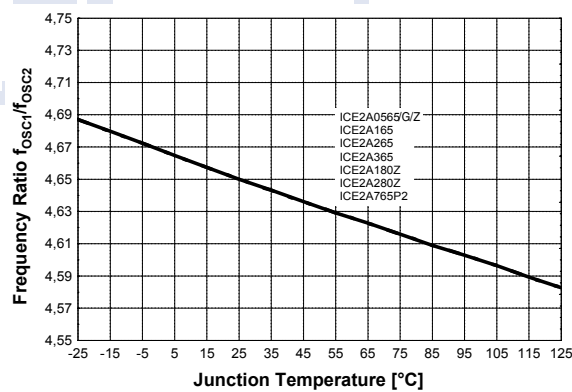
Figure 39 Frequency Ratio f_{OSC1}/f_{OSC2} vs. T_j
