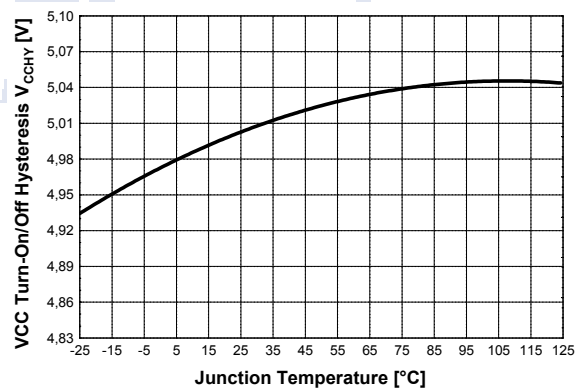
Figure 33 VCC Turn-On/Off Hysteresis V_{VCHY} vs. T_j
