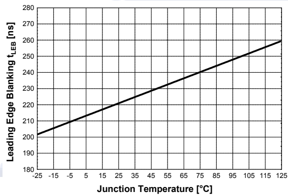
Figure 50 Leading Edge Blanking V_{CC1} vs. T_j
