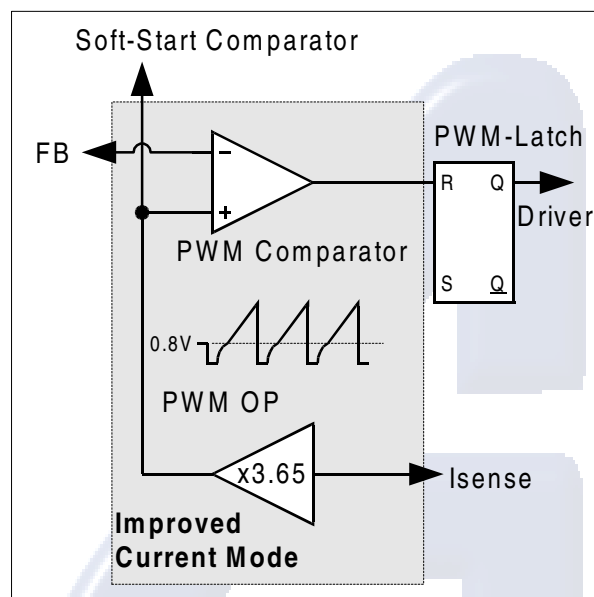
Figure 7 Current Mode
