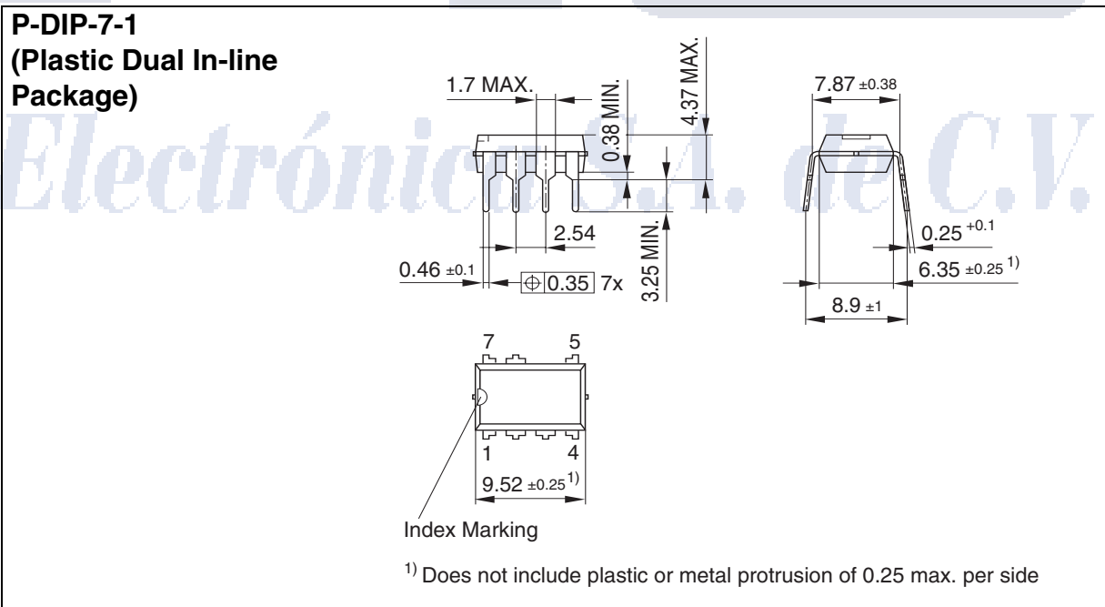
Figure 59 P-DIP-7-1 (Plastic Dual In-line Package)
