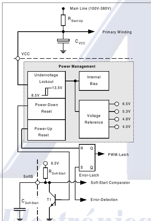
Figure 6 Power Management
