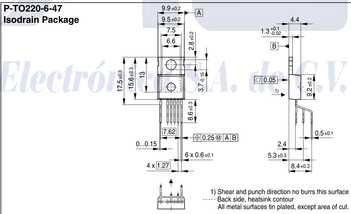
Figure 61 P-TO220-6-47 (Isodrain Package)
