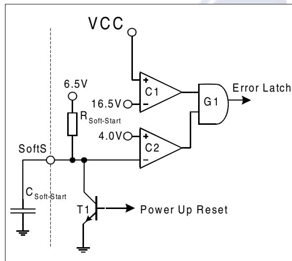
Figure 24 Overvoltage Detection
