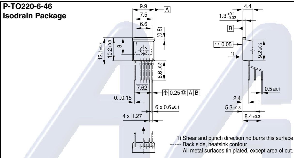
Figure 60 P-TO220-6-46 (Isodrain Package)
