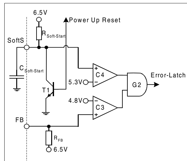
Figure 22 FB-Detection
