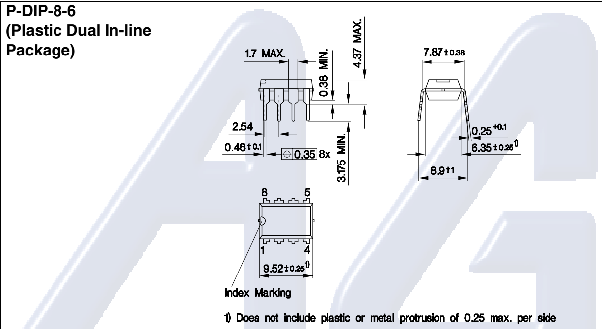
Figure 58 P-DIP-8-6 (Plastic Dual In-line Package)
