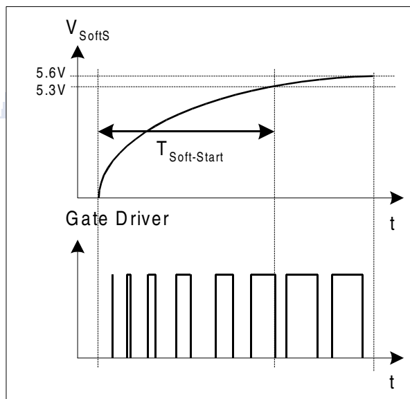
Figure 12 Soft-Start Phase
