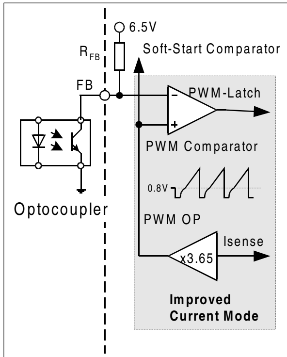
Figure 11 PWM Controlling
