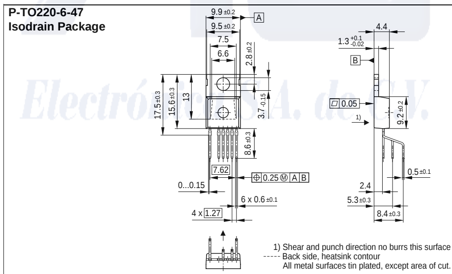
Figure 60 P-TO220-6-47 (Isodrain Package)
