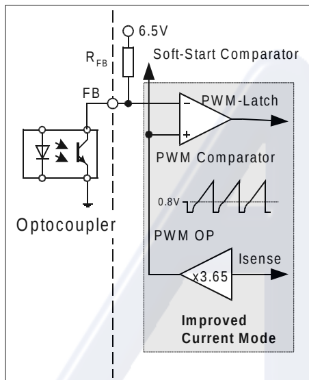
Figure 10 PWM Controlling
