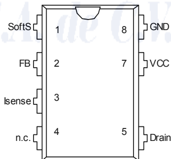
Figure 2 Pin Configuration (top view)
