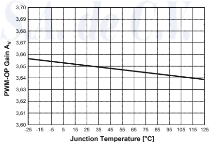
Figure 41 PWM-OP Gain A_v vs. T_j
