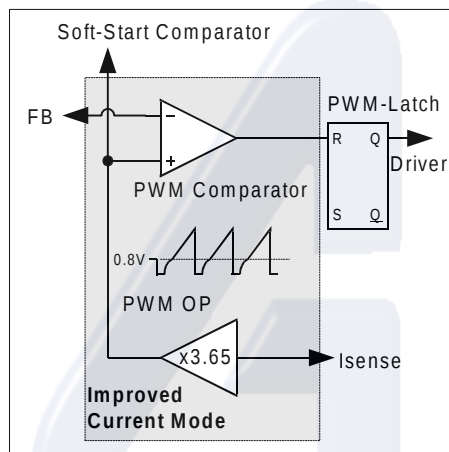
Figure 6 Current Mode
