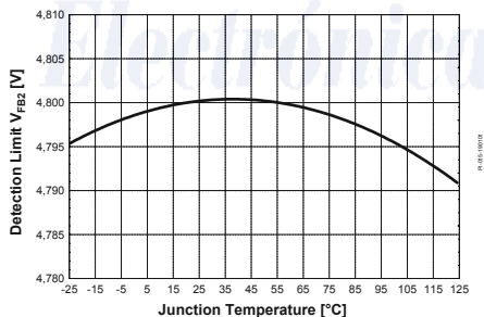
Figure 44 Detection Limit V_{FB2} vs. T_J
