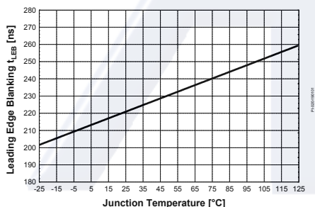
Figure 49 Leading Edge Blanking V_{VCC1} vs. T_j
