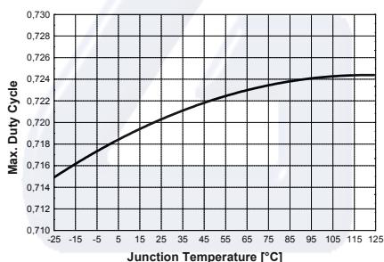
Figure 40 Max. Duty Cycle vs. T_j
