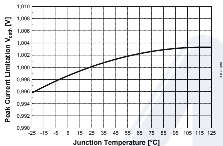
Figure 48 Peak Current Limitation V_{csth} vs. T_j
