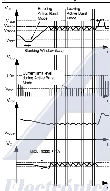
Figure 8 Signals in Active Burst Mode
