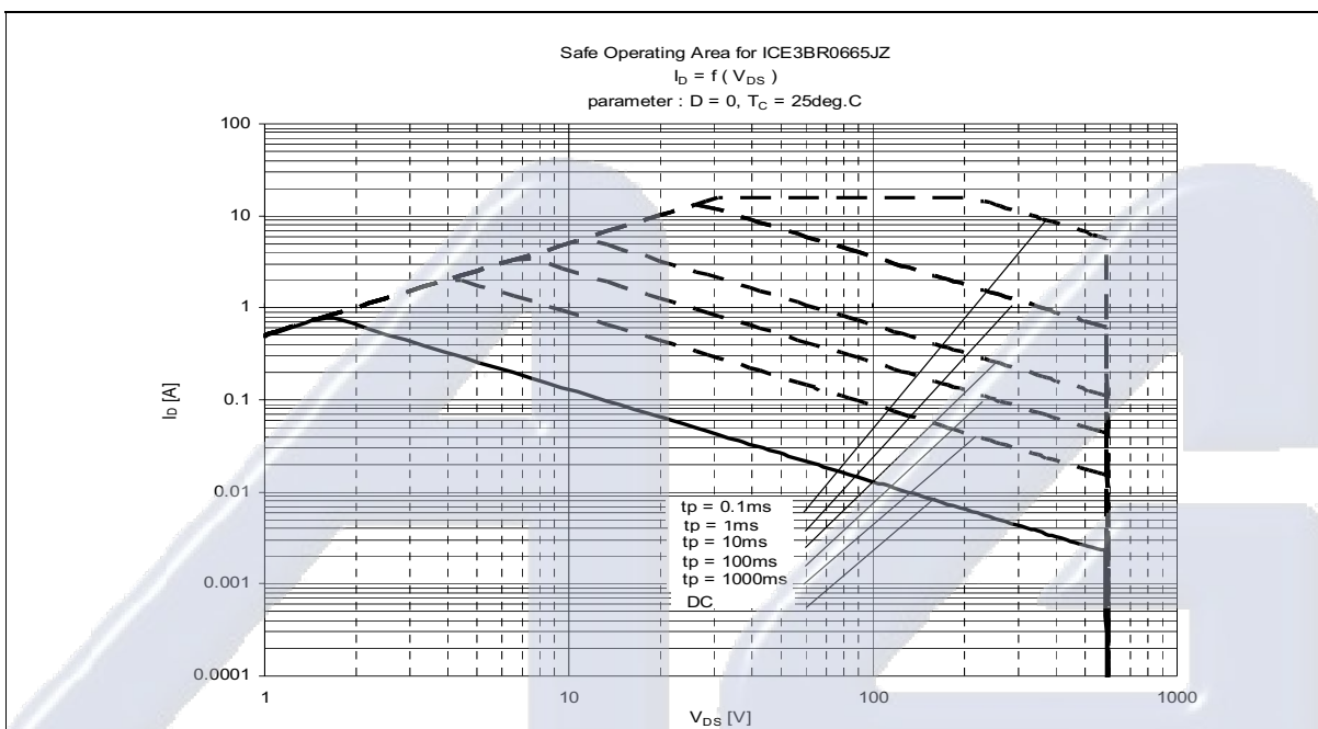
Figure 27 Safe Operating Area (SOA) curve for ICE3BR0665JZ
