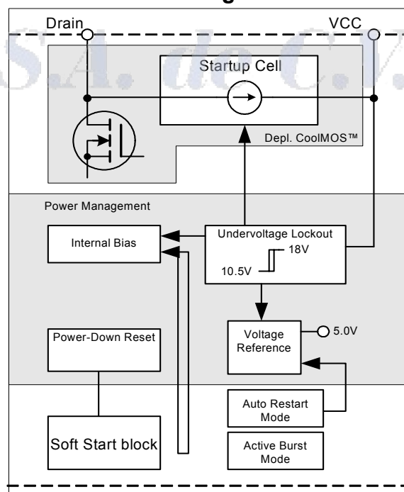
Figure 3 Power Management
