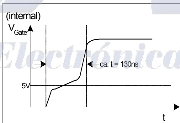
Figure 16 Gate Rising Slope
