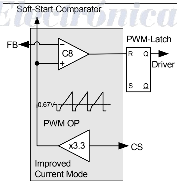
Figure 4 Current Mode
