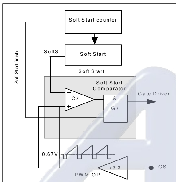
Figure 9 Soft Start
