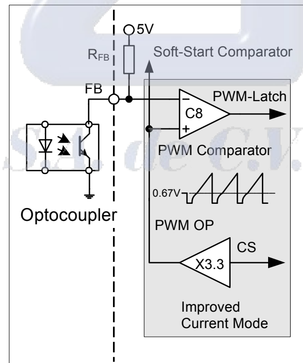
Figure 8 PWM Controlling
