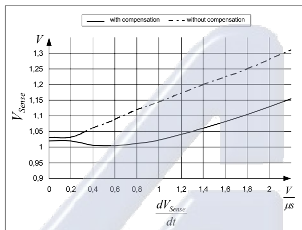
Figure 20 Overcurrent Shutdown
